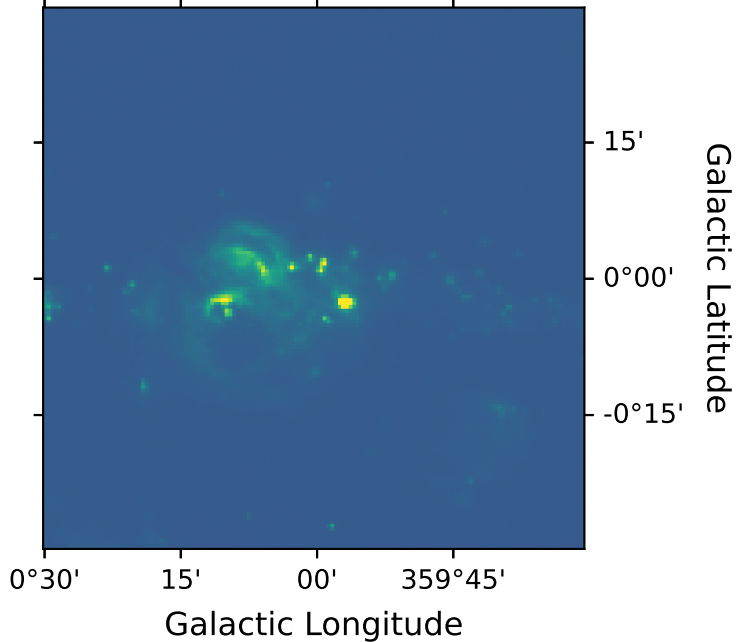
MSX band E
