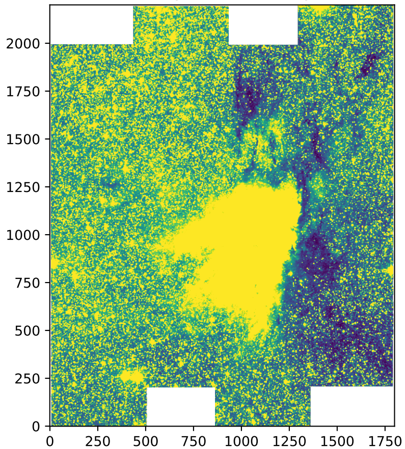
Background matching
