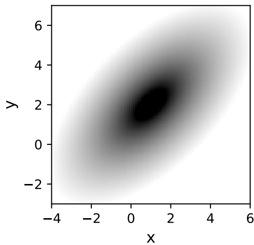
Sersic2D
