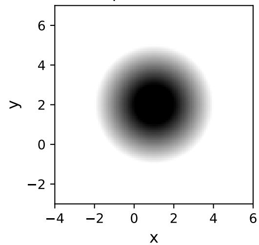
TrapezoidDisk2D
