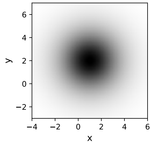
Moffat2D
