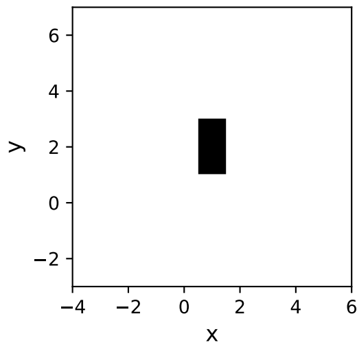
Box2D
