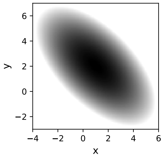
Gaussian2D
