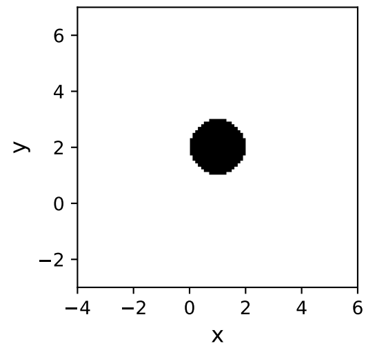
Disk2D
