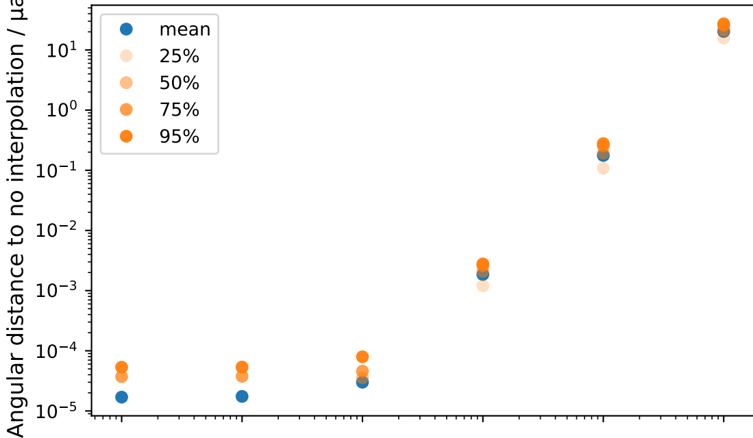
Transformation of SkyCoord with 100.000 obstimes over 12 hours
