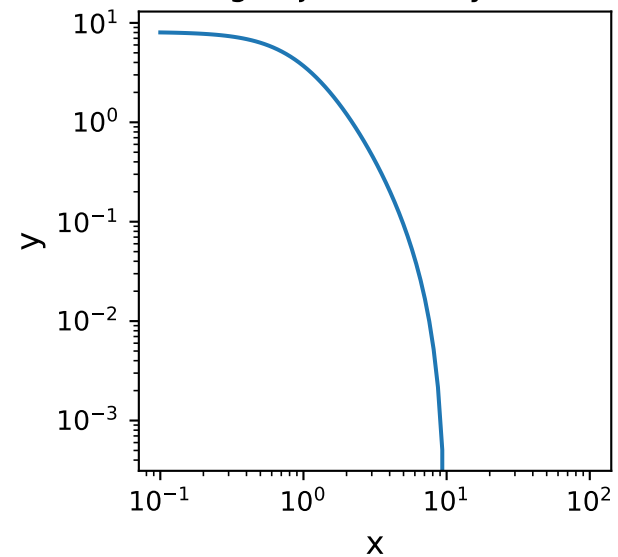
KingProjectedAnalytic1D
