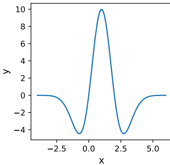
RickerWavelet1D
