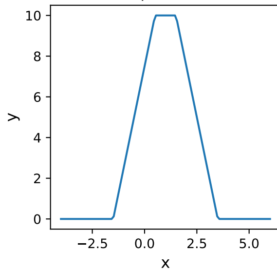
Trapezoid1D
