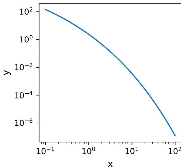
Sersic1D
