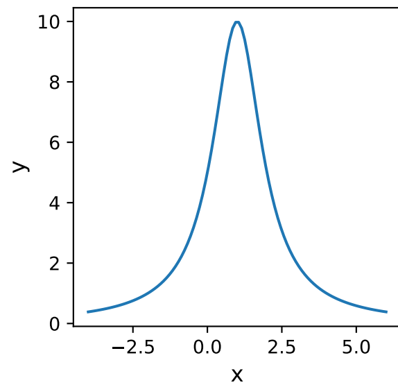
Moffat1D
