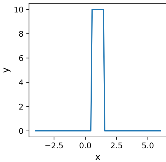
Box1D
