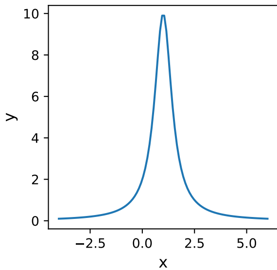
Lorentz1D
