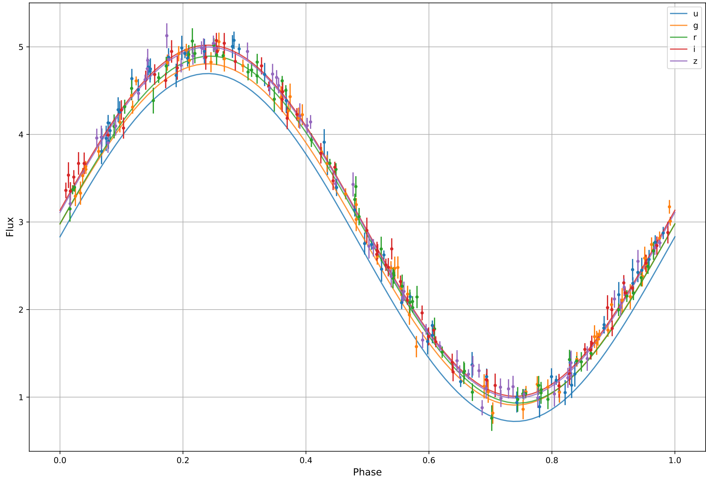
Multiband Phase Model
