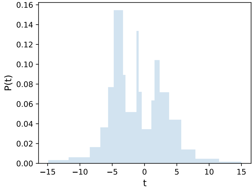
hist(t, bins="blocks")
