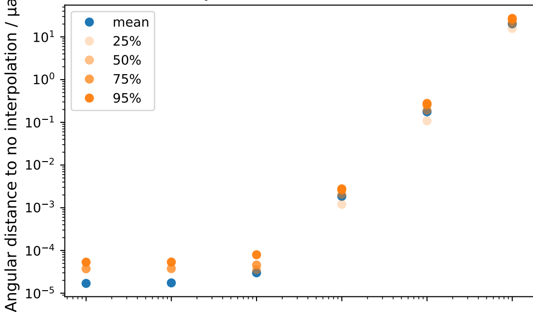
Transformation of SkyCoord with 100.000 obstimes over 12 hours
