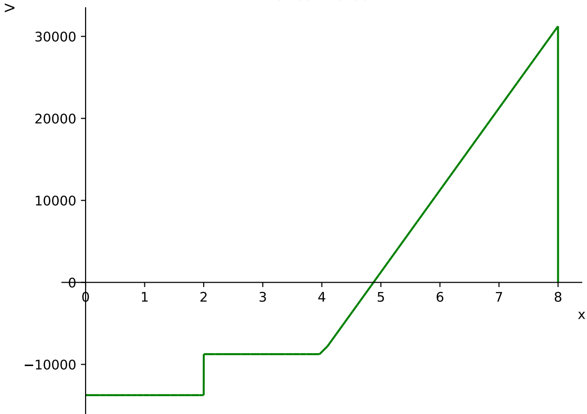
Shear Force
