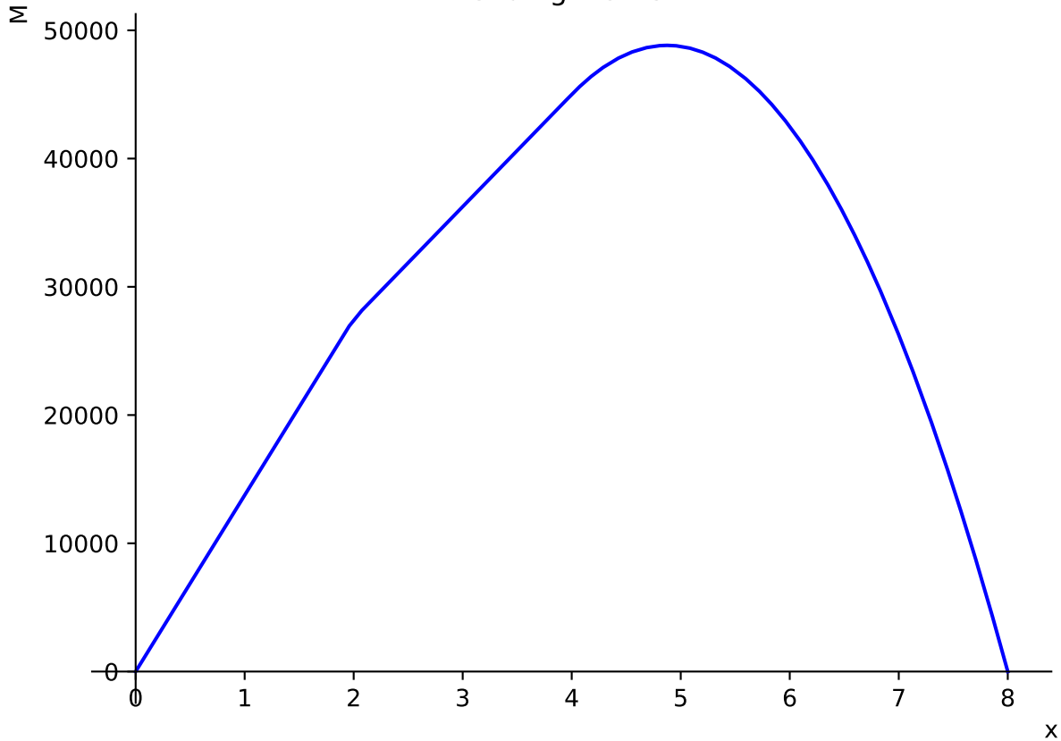
Bending Moment
